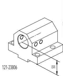
Toolholder for insertdrill with internal coolant Ø40 mm
